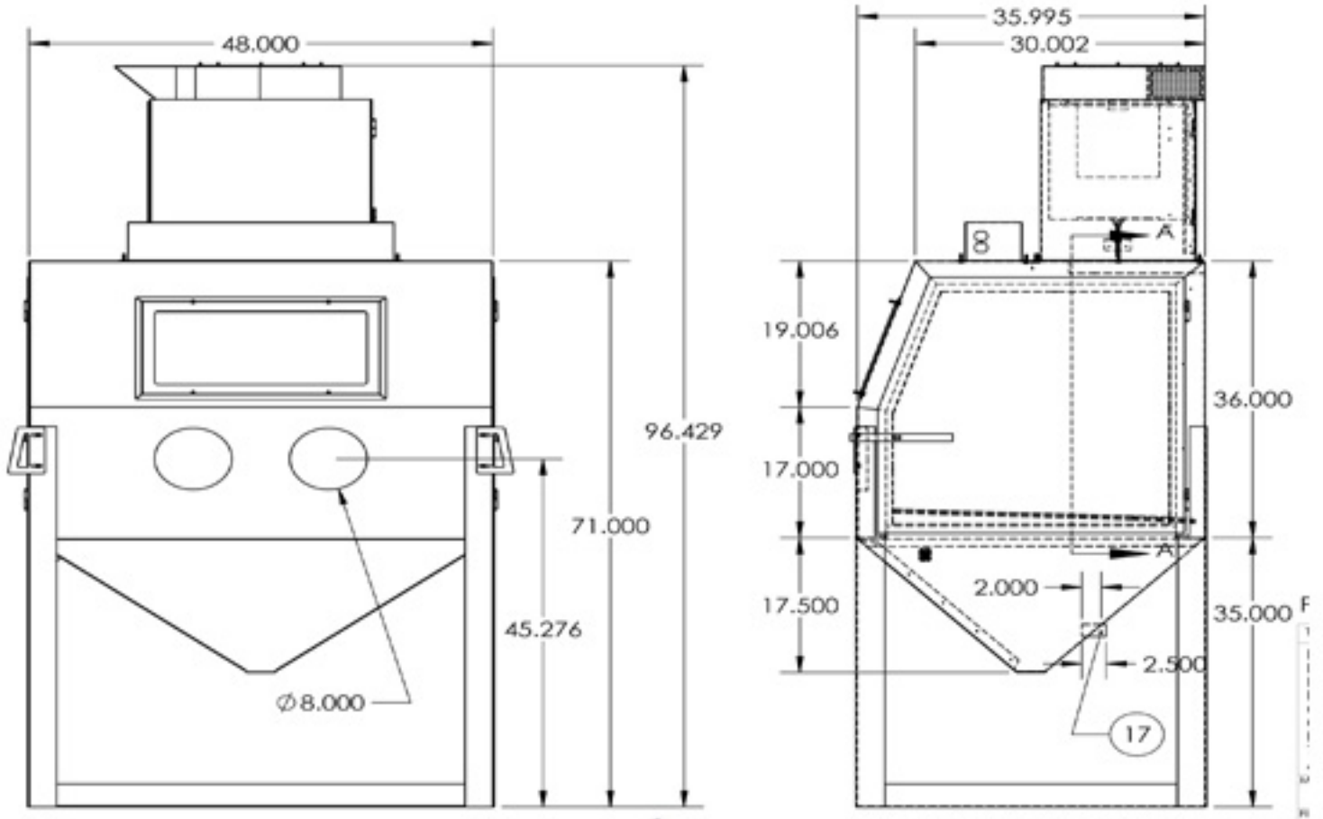
Vapor King shown with Graco EQp
